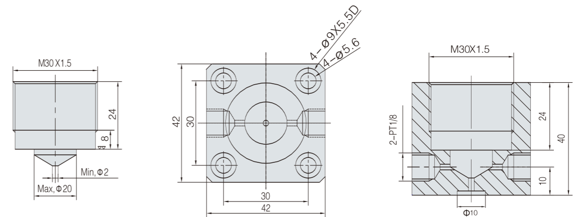
安裝底座示意圖 Schematic diagram of mounting base
