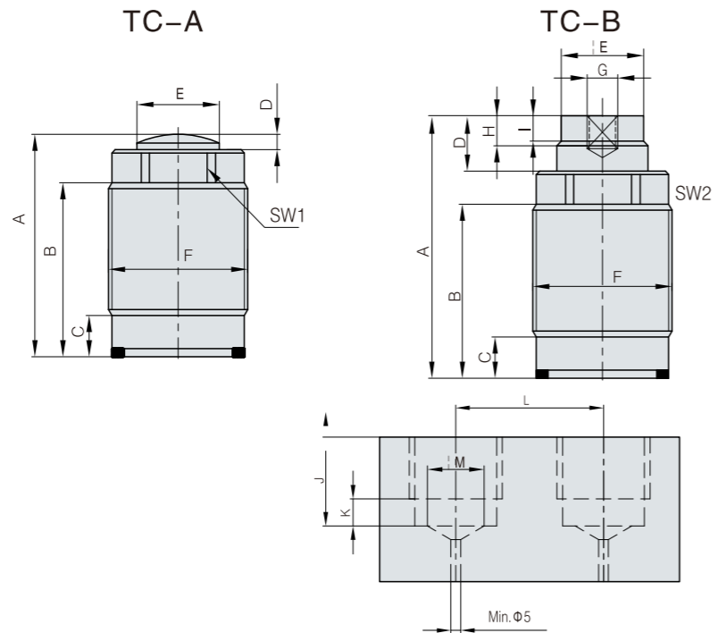
安裝底座示意圖 Schematic diagram of mounting base
